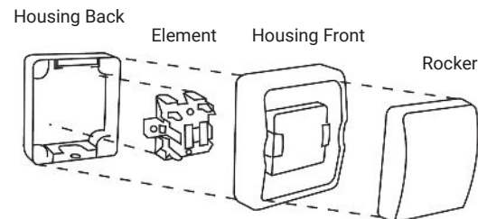
Figure 1 | Way Switch Figure 2 | Change-over switch
